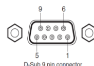
D-Sub 9 pin connector
